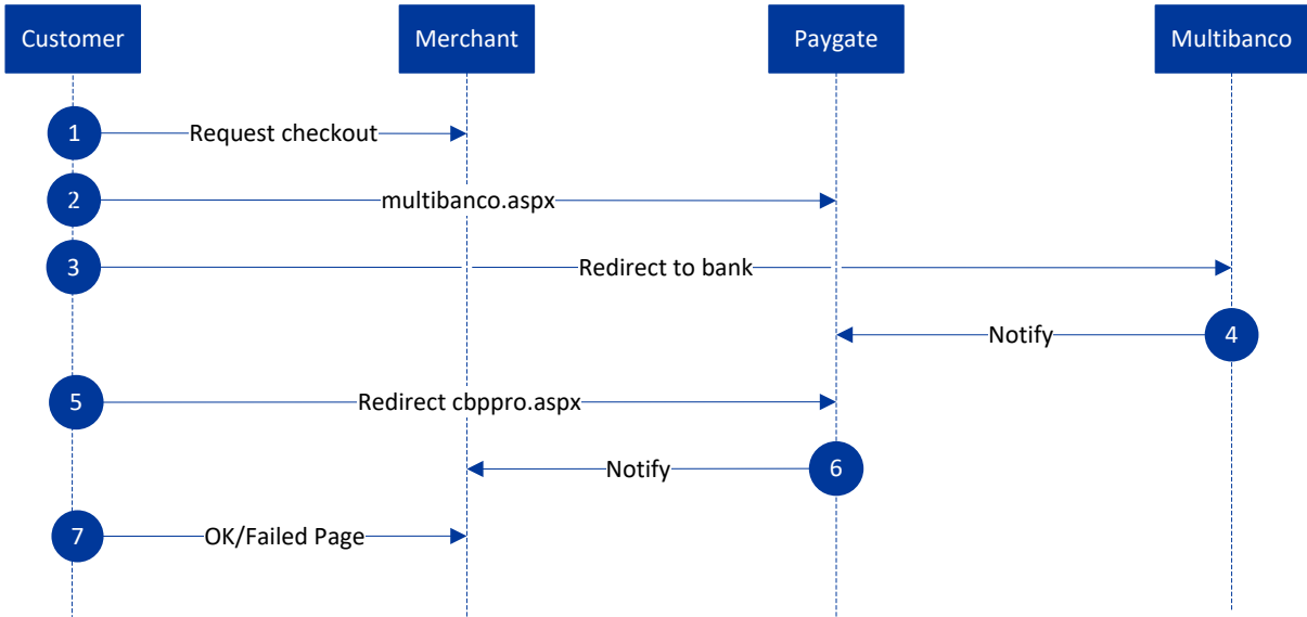
Multibanco process flow
