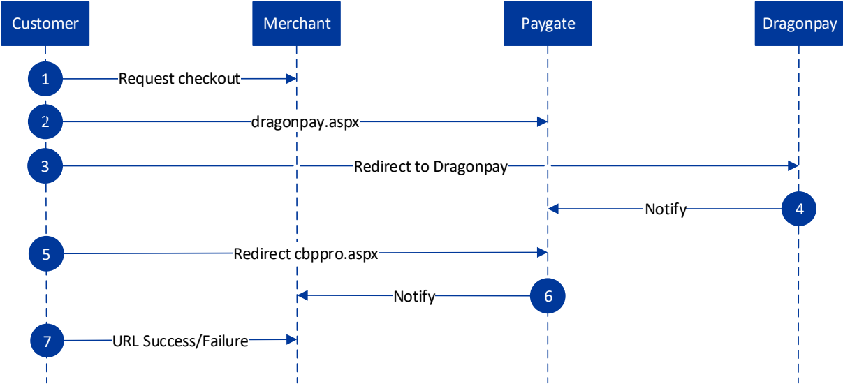
Dragonpay process flow
